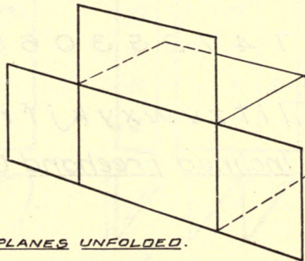
3rd. ANGLE OF PROJECTION, SHOWING THE VERTICAL AND HORIZONTAL PLANES.
